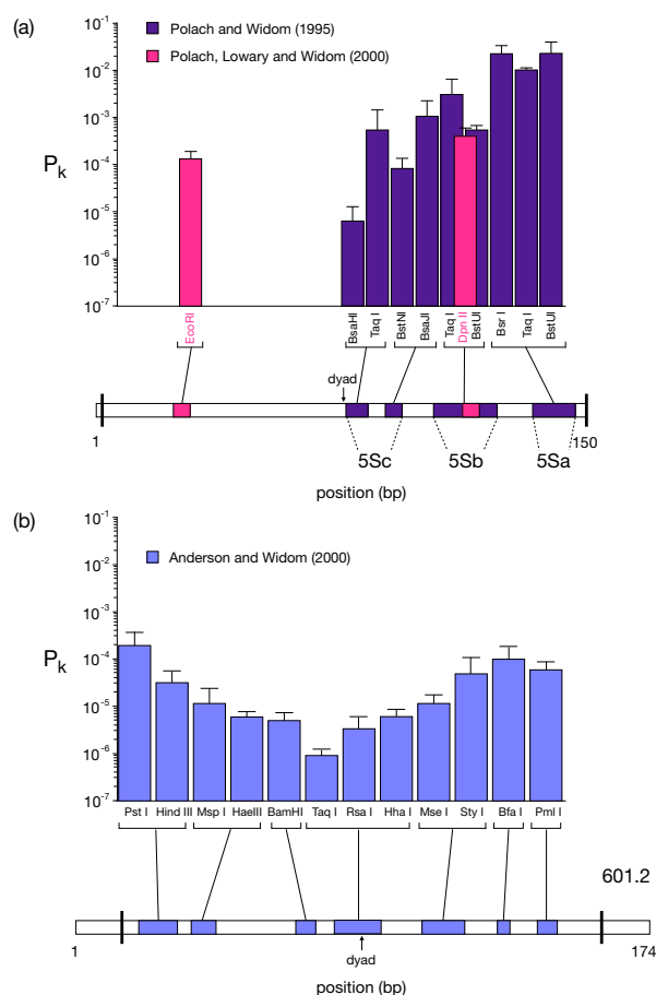
Fig. 7. Results of restriction enzyme experiments on nucleosome breathing, carried out by the Widom lab [17–19]. Accessibility profiles for (a) the 5S nucleosome [17, 19] and (b) the 601 nucleosome [18]. Below the plots are schematic depictions of the DNA molecules used in the experiments. Coloured stretches indicate the positions of the restriction sites and the black vertical bars indicate the edges of the regions occupied by the nucleosome. Note the non-monotonic decay in accessibility, which is most likely due to the use of different restriction enzymes (which have different shapes and sizes and require different salt concentrations and temperatures) and the varying orientations of the restriction sites with respect to the octamer.
